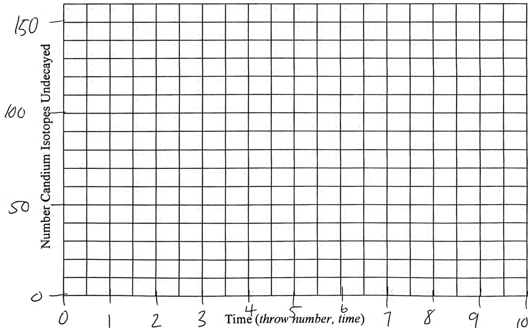
Graph of decayed particles over time to find the half-life of candium isotopes
